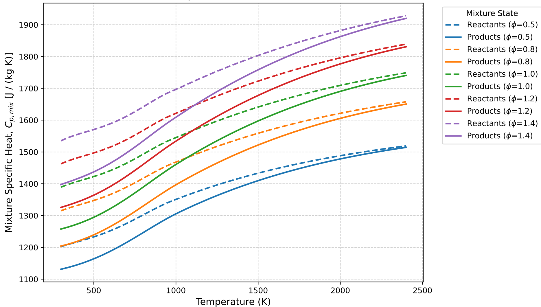
Variation of Mixture C_p for Hydrogen ( H_2 )-Air (Frozen Products)
